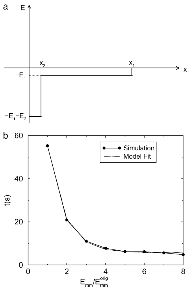
FIGURE 9 Two-step potential well model (a) and fitting results (b) for L = 25 using Eq. 25. The fit parameters are t_\infty = 5.68 s, t_0 = 162.2 s, and E_d = 0.87 E_{mm}^{ion} .
