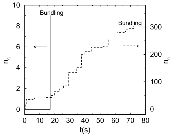
FIGURE 2 Number of collisions n_c before time t for two simulation trajectories. (Solid line) E_{mm} = 8E_{mm}^{\text{ion}} ; (dotted line) E_{mm} = E_{mm}^{\text{ion}} . L = 25 for both lines. Their lowest interaction energies are -0.269 eV ( -10.4 kT) and -2.15 eV ( -83.1 kT), respectively.
