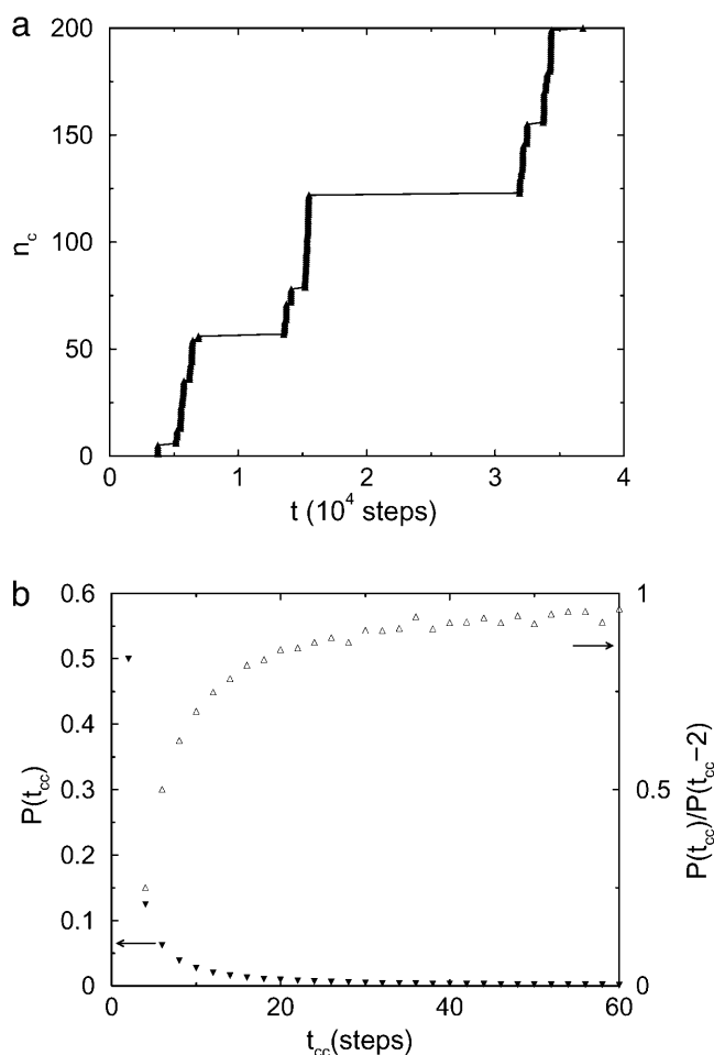
FIGURE 10 (a) Number of collisions n_c before time t , in which solid triangles show times of the first 200 sequential collisions in a simulation trajectory with X_m = 100 and 10^9 steps; (b) probability distribution P(t_{cc}) of t_{cc} , the time spacing between two successive collisions, in the same simulation trajectory. Note that probability of odd t_{cc} is zero. For large, even t_{cc} values, the probabilities are close to zero, but are not zero. Probabilities of t_{cc} values > 60 steps are not shown. Open triangles in b are probability ratios.
