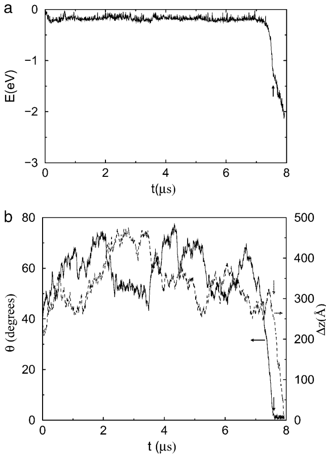
FIGURE 6 Bundling for strong attraction E_{mm} = 8E_{mm}^{\text{ion}} and L = 25 . (a) Energy during last collision, which leads to bundling. The value t = 0 is the beginning time for this collision. (b) Angle \theta (solid line) and displacement \Delta z along the z axis between the centers of two filaments (dotted line) during the last collision. Downward arrows mark separation of the rotation and sliding phases of bundling.
