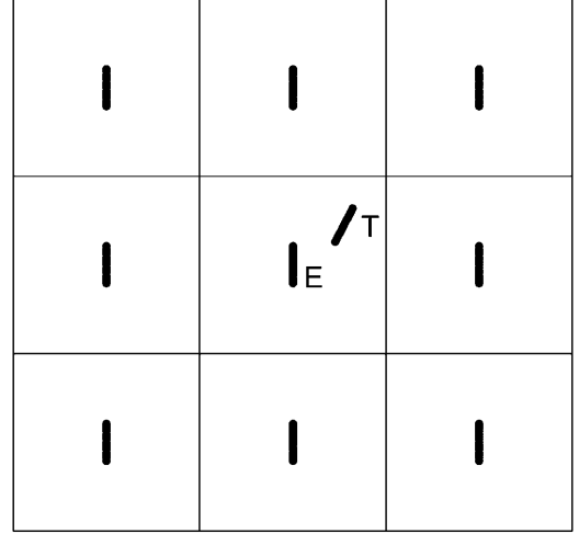
FIGURE 1 The Brownian dynamics simulations are carried out under periodic boundary conditions, with variable time steps. One filament is chosen as the target (marked T ), which moves through other environmental filaments (marked E ), centered in cells. Environmental filaments are frozen; target filament moves relative to the environmental filament at the center of its cell.
