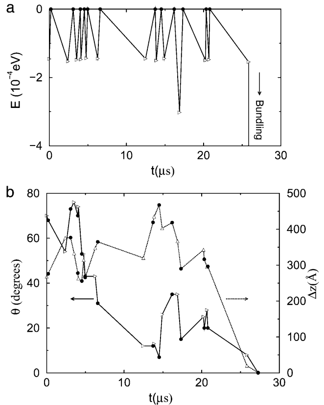
FIGURE 7 Bundling for weak attraction E_{mm} = E_{mm}^{\text{ion}} and L = 25 . Energy (a), angle \theta (b, solid line), and z -displacement \Delta z (b, dotted line) during last encounter. (Open triangles) Collisions begin; (solid circles) collisions end. Last collision leads to bundling.
